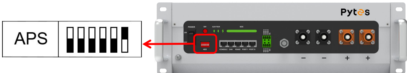
Figure 1.1.4 APS DIP switch setting
